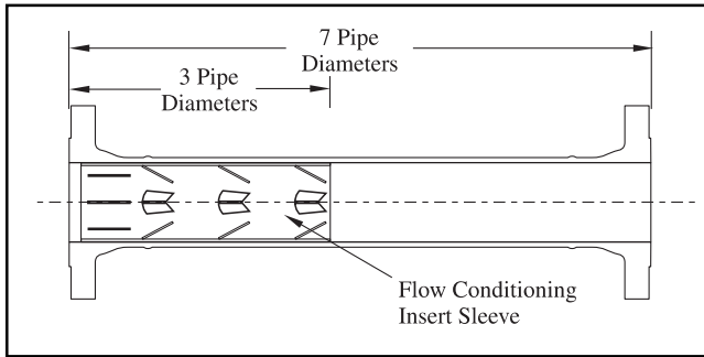
Figure 11 — High Performance Flow Conditioner
