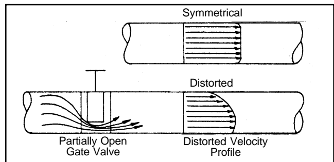
Figure 6 — Velocity Profile Distortion After Gate Valve
