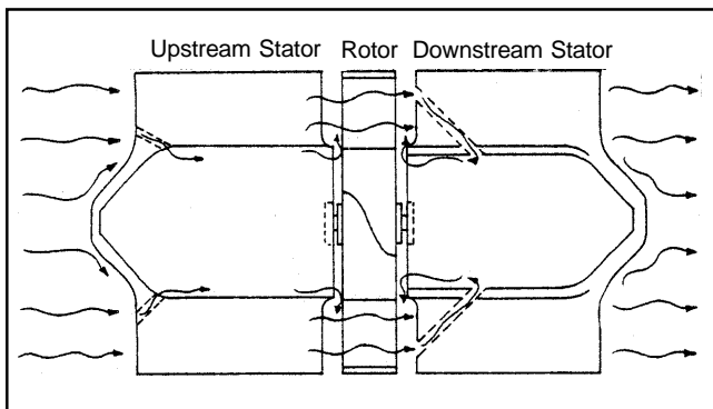
Figure 9 — Floating Rotor - Smith Sentry turbine meter
