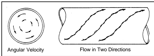
Figure 7— Effect of Fluid “Swirl”
