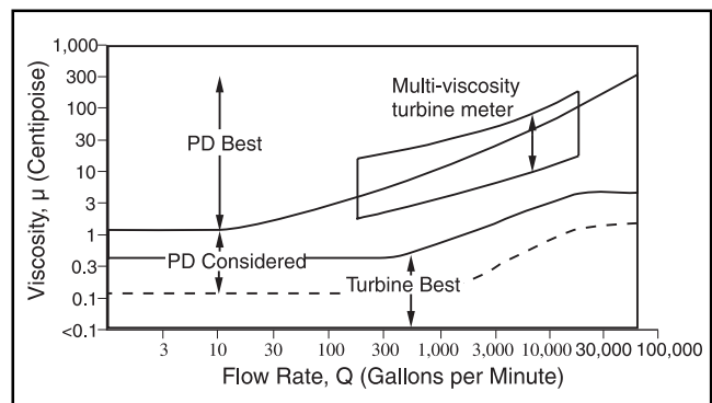
Figure 10 — Meter Application Ranges
