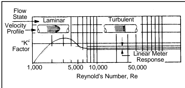
Figure 4 — Universal Turbine Meter Performance Curve
