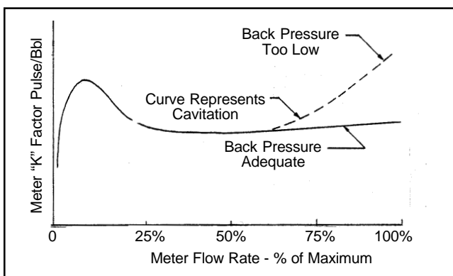
Figure 5 — TM Performance with Cavitation
