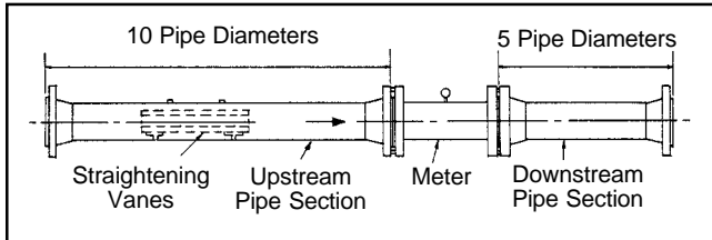
Figure 8 — API Recommended Flow Conditioning
