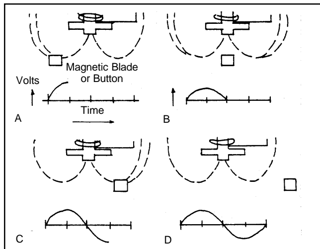
Figure 2 — Principle of Reluctance Signal Generation
